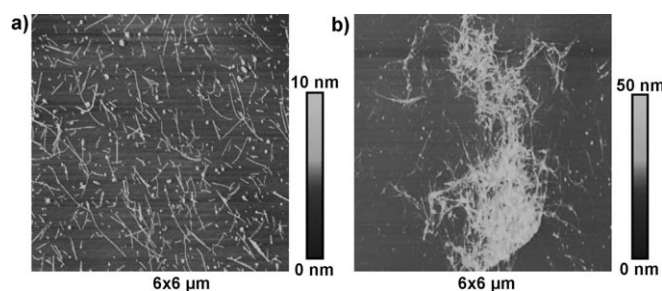
Figure 3. AFM images of the DNA-conjugated SWNT-[1,3] a) before and b) after hybridization with SWNT-[1,4]. See Figures S3 and S4 in the Supporting Information for more AFM images showing the aggregated and dispersed SWNT samples.
